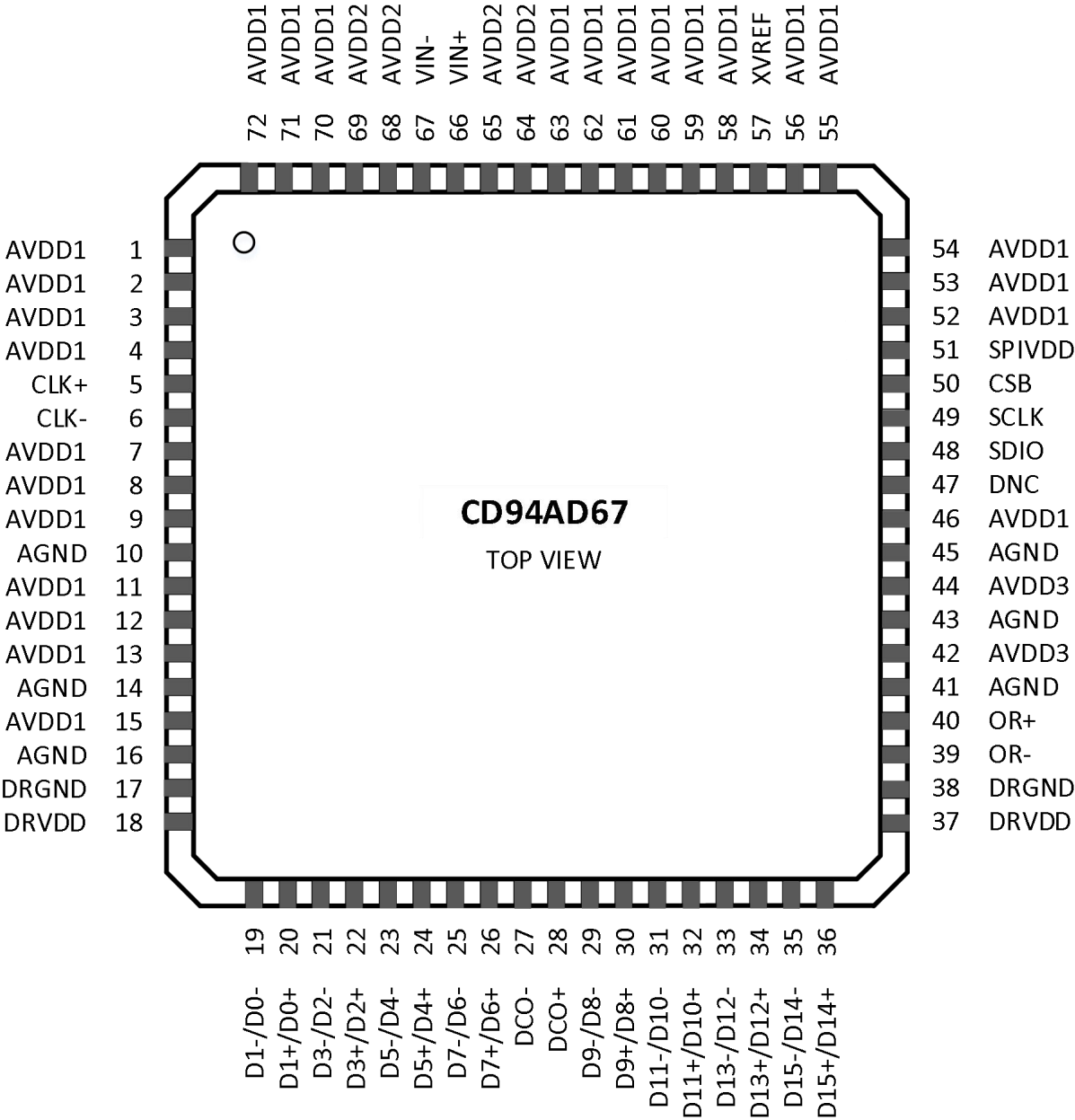
CD94AD67 Pin Configuration
