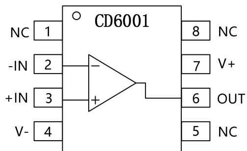
SOP-8
