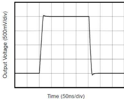
Non-Inverting Large-Signal Step Response
