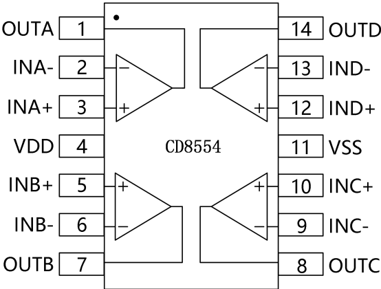
SOP-14 / TSSOP-14
