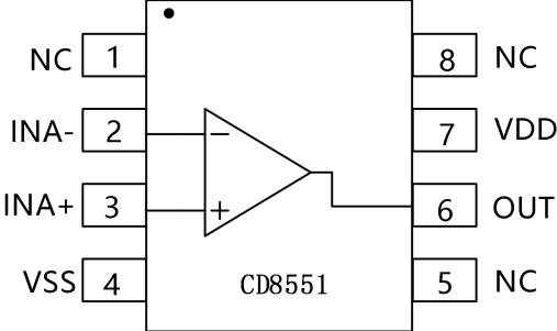
SOP-8
