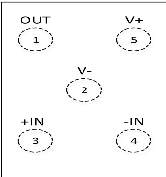
CD8605 (TOP VIEW)
