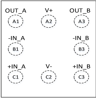
CD8606 (TOP VIEW)
