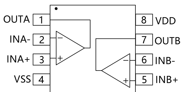
SOIC-8(SOP8),MSOP-8,TDFN2x2-8
