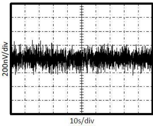
0.01Hz TO 1Hz NOISE AT Vs=2.7V
