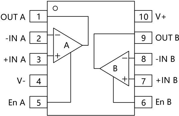
MSOP-10
