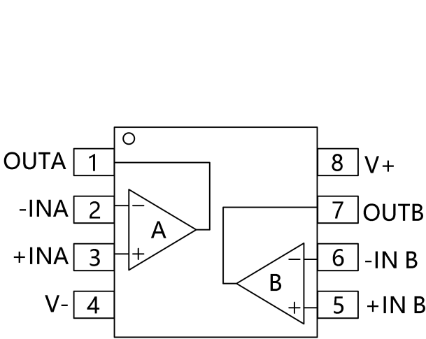
SOIC-8(SOP8),MSOP-8,TSSOP-8 TDFN2x2-8L,TDFN3x3-8L
