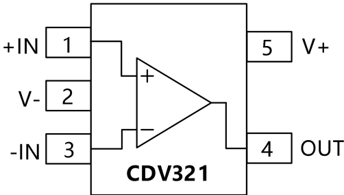
SOT23-5 (AST5)
