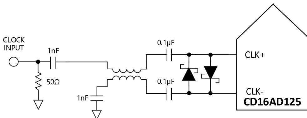
Figure 18. Balun configured clock
