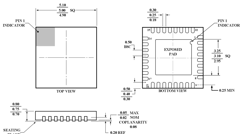
Figure 3. Package Outline Dimensions
