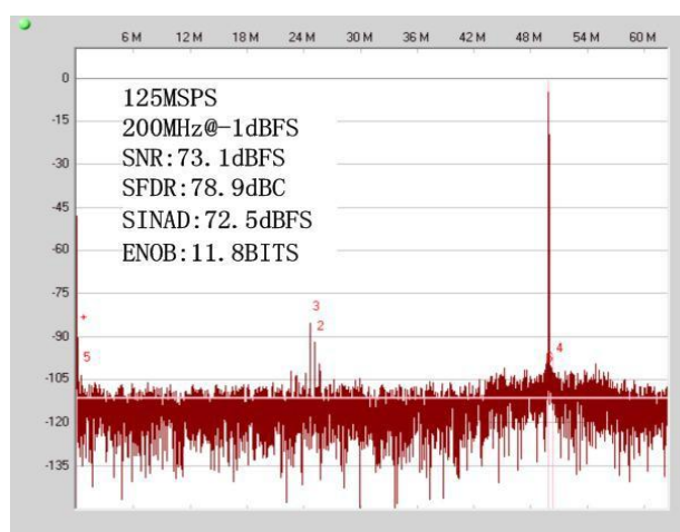
Figure 10. Single-Tone FFT with f_{IN} = 200\text{MHz}
