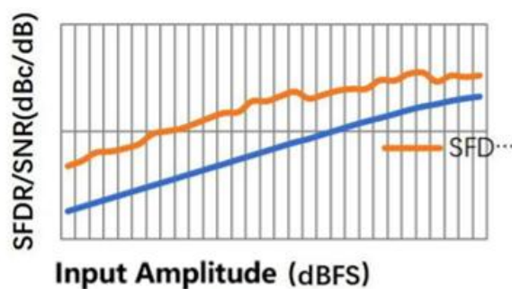
Figure 12 SNR/SFDR vs. Input Amplitude ( f_{in}=70\text{MHz} , Dither Off)
