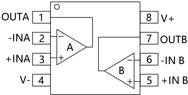
SOIC-8(SOP8),MSOP-8,TSSOP-8 TDFN2x2-8L,TDFN3x3-8L
