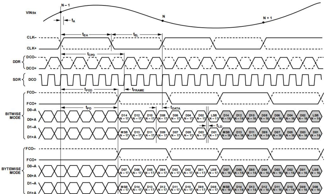
Figure 3. 16-Bit DDR/SDR, Two-Lane, 1 × Frame Mode (Default)
