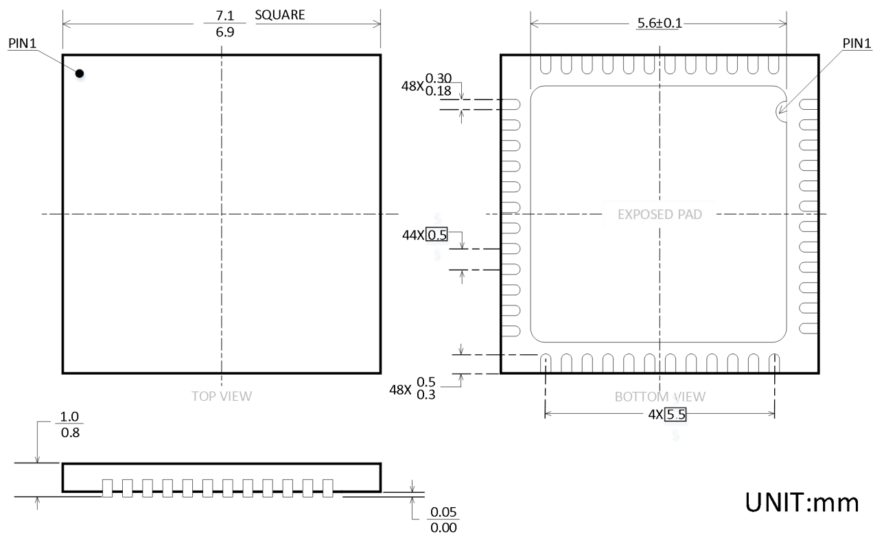
Figure 17. QFN-48 Packaging Dimensions
