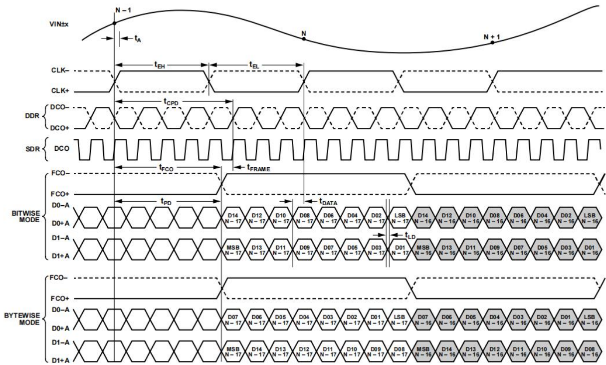
Figure 3. 16-Bit DDR/SDR, Two-Lane, 1 × Frame Mode (Default)
