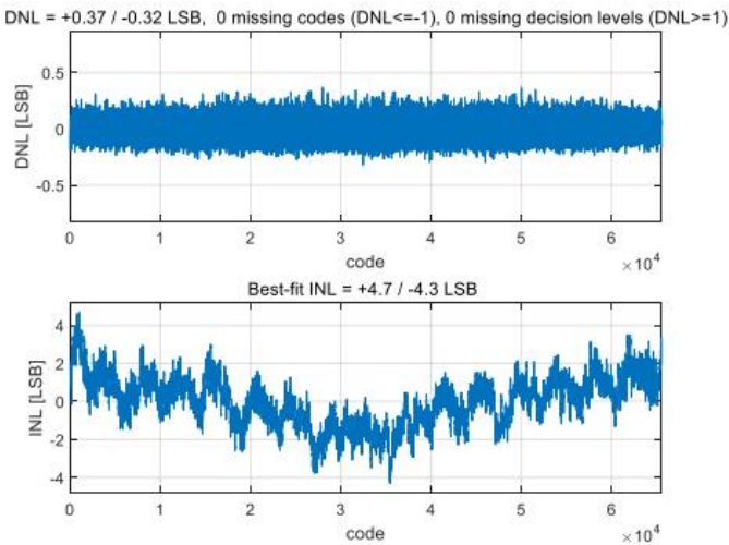
Figure 11.DNL/INL(fin=10MHz, fS=125MSPS)
