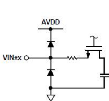
Figure 7. Equivalent Analog Input Circuit
