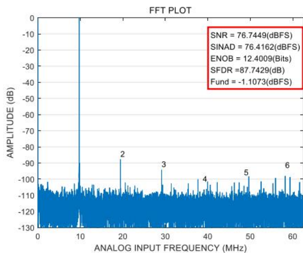
Figure 7. Single-tone 32K (fIN=10MHz, fS=125MSPS)
