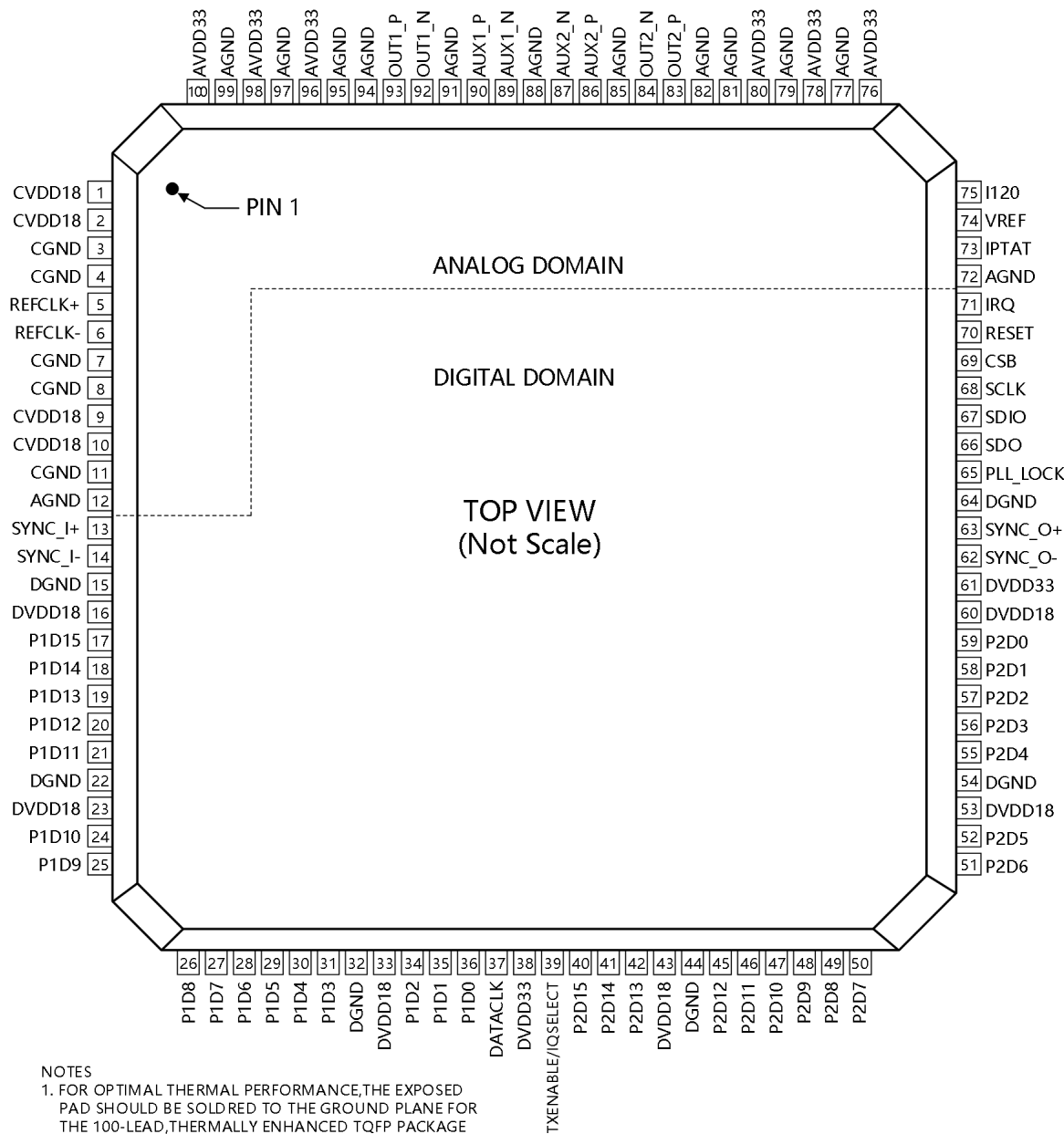
Figure 2. Pin Arrangement Diagram
