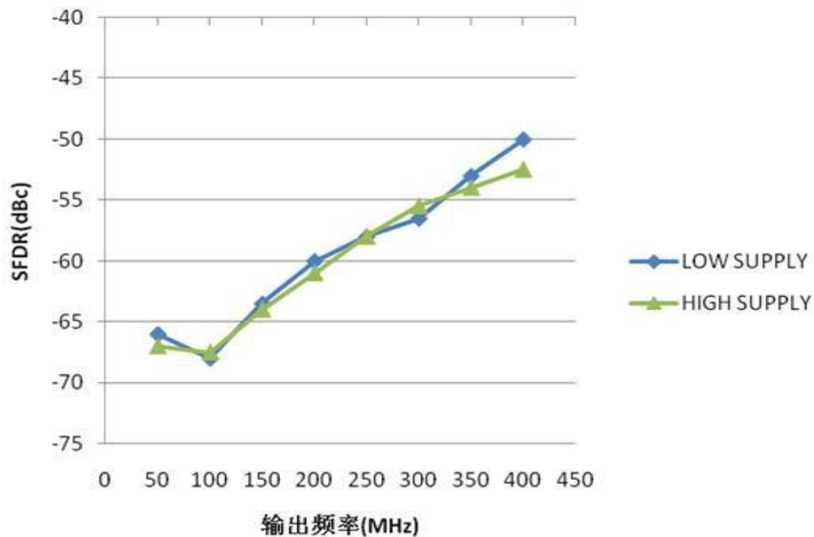
Figure 10. Wideband SFDR Output Frequency vs. Supply (±5%), REFCLK = 1 GHz
