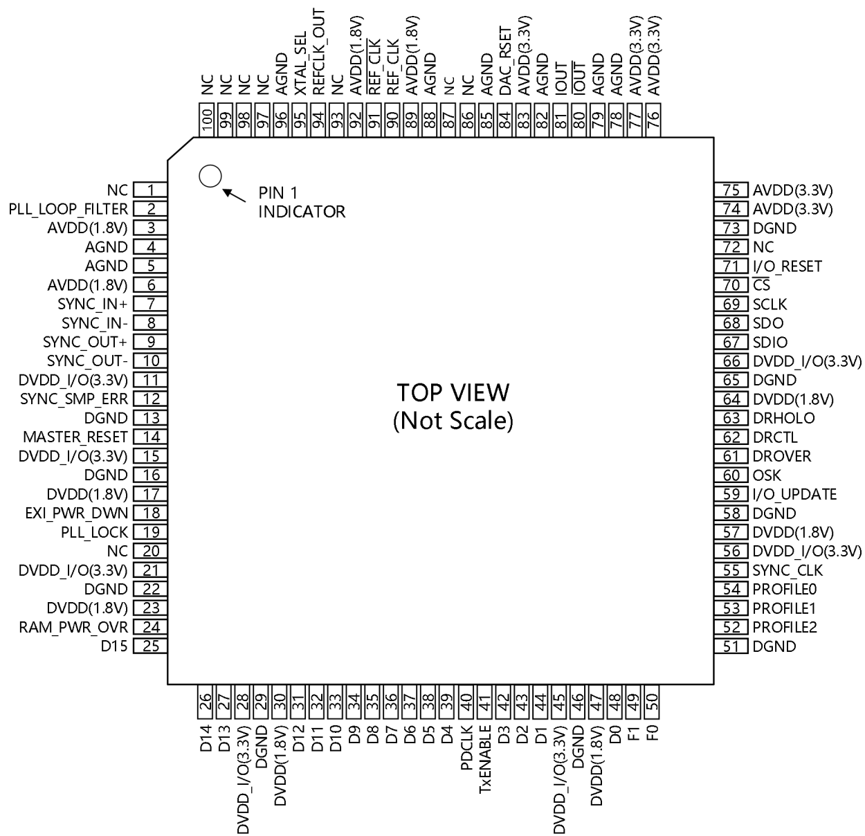
Figure 2. Pin Configuration
