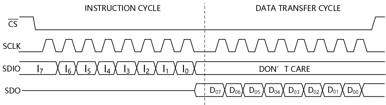
Figure 15. 3-Wire Serial Port Read Timing—Clock Stall Low
