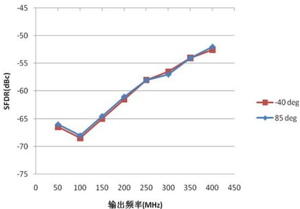
Figure 11. SFDR vs. Frequency and Temperature in Single Tone Mode, REFCLK = 1 GHz
