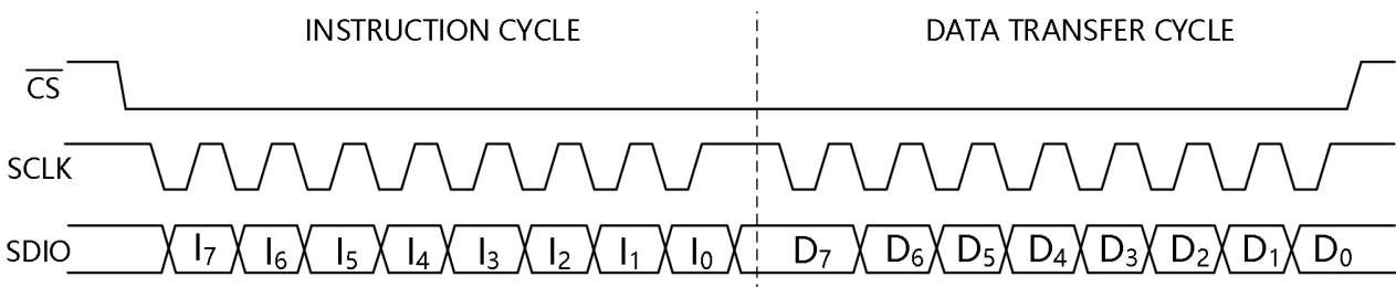
Figure 16. Serial Port Write Timing—Clock Stall High
