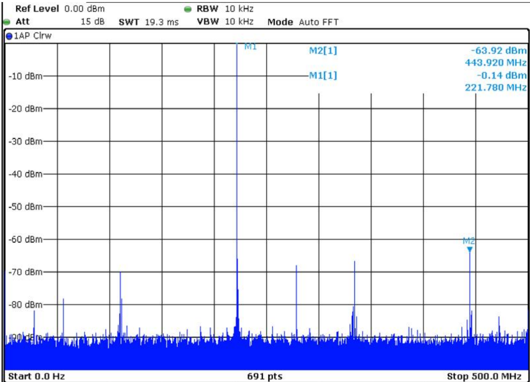
Figure 4. 15.625 kHz Quadrature Tone, Carrier = 222.1 MHz, CCI = 16, f_s = 1 GHz
