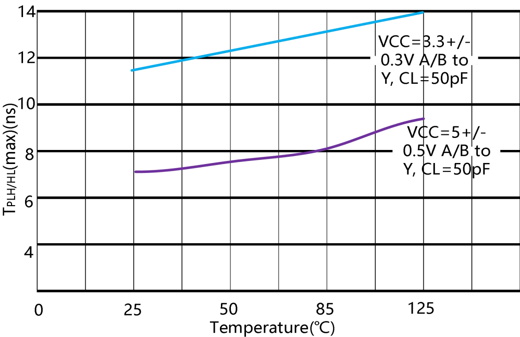
Figure 3.Propagation Delay vs Temperature
