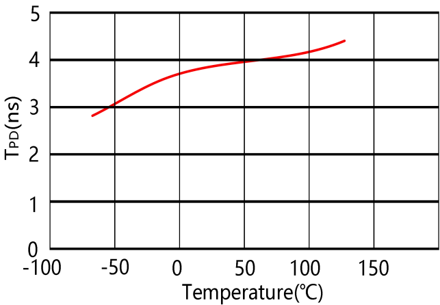
Figure 3. T_{PD} vs Temperature
