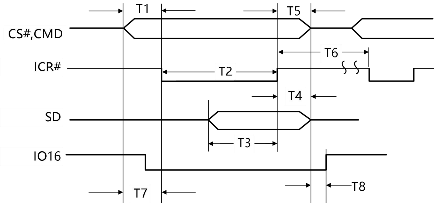
Figure 5. Processor Write Timing
