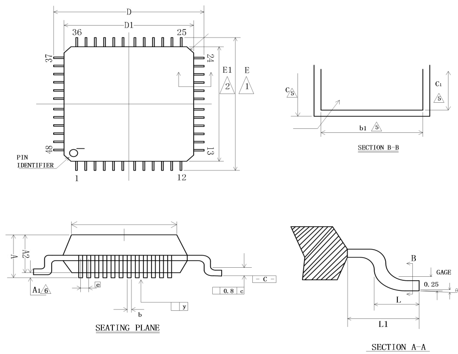
Figure 9. 48-Lead Outline Package [TQFP]
