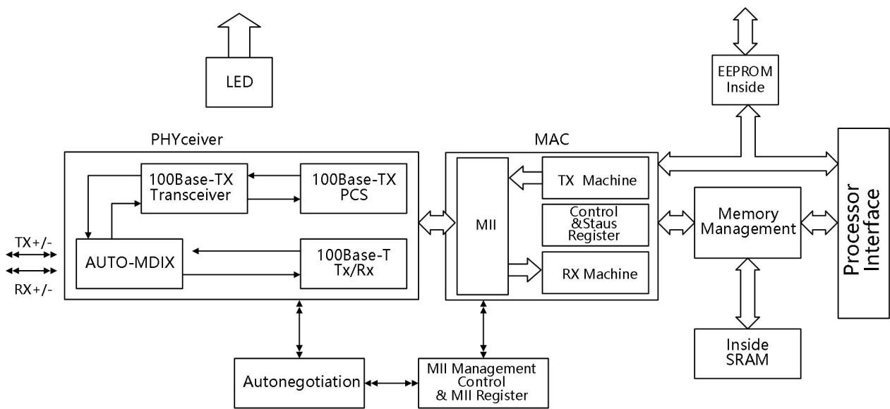
Figure 1. Block Diagram
