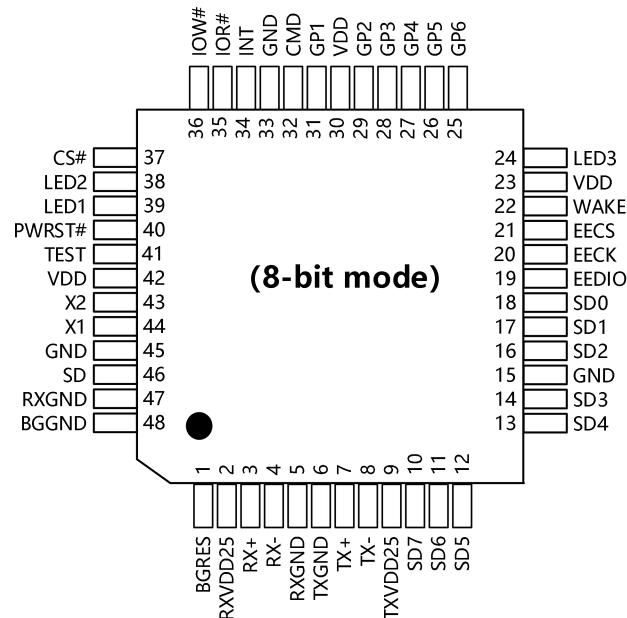
Figure 3. 8-bit mode
