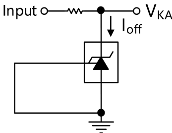
Figure 3. Test Circuit for I_{off}
