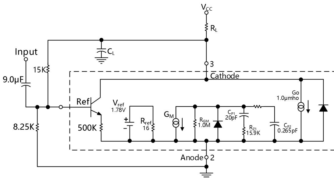
Figure 31. Simplified CD432 Device Model
