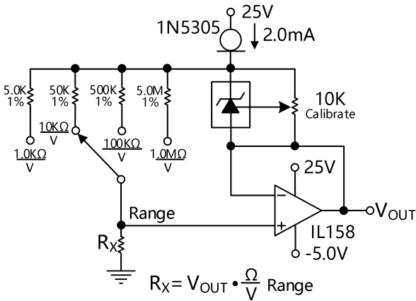
Figure 28. Linear Ohmmeter
