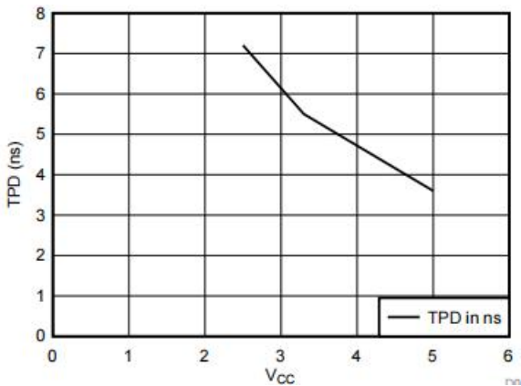
Figure 3.TPD vs VCC at 25°C
