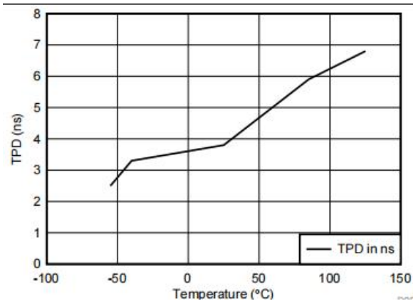
Figure 3.TPD vs Temperature
