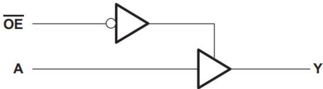
Figure 2. Functional Block Diagram
