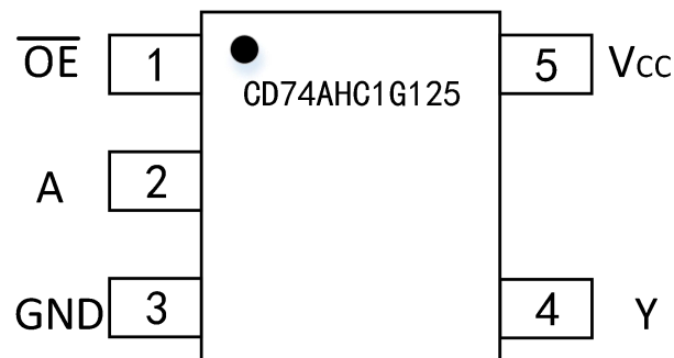
Figure 1. SOT23-5 Pin Configuration
