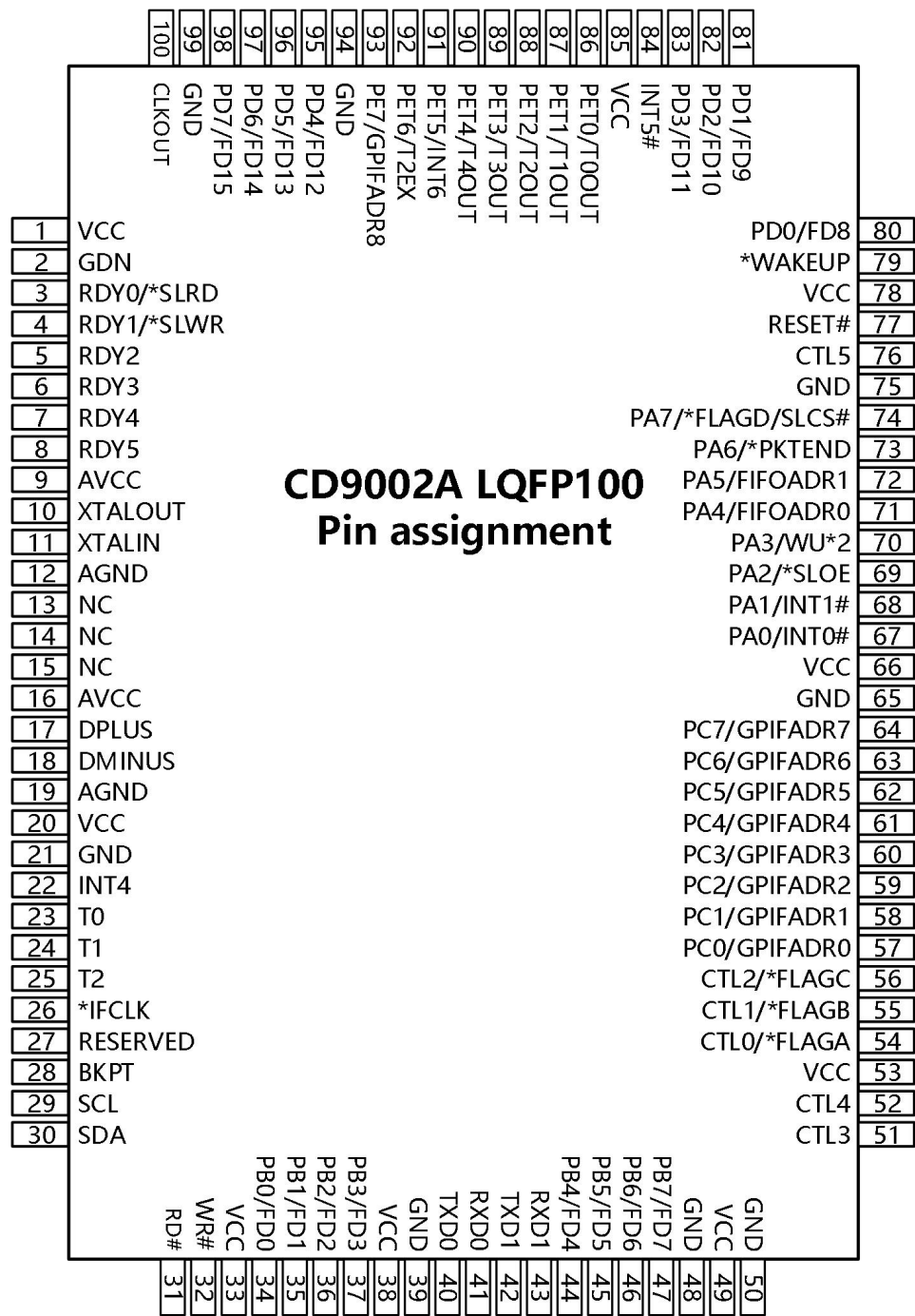
Figure 2. CD9002A LQFP100 pin assignment
