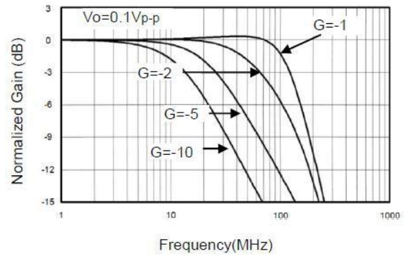
Inverting Small Signal Frequency Response
