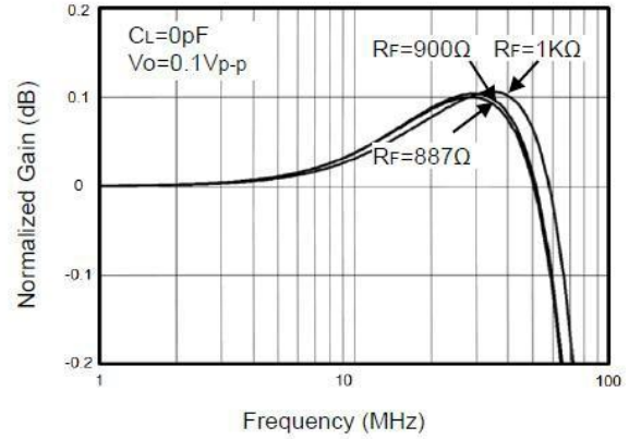
0.1dB Gain Flatness For Various R_F
