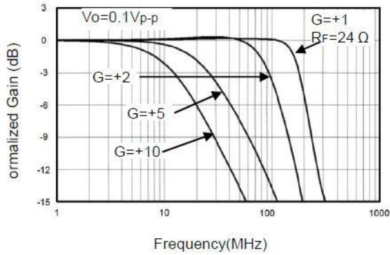
Non-Inverting Small Signal Frequency Response
