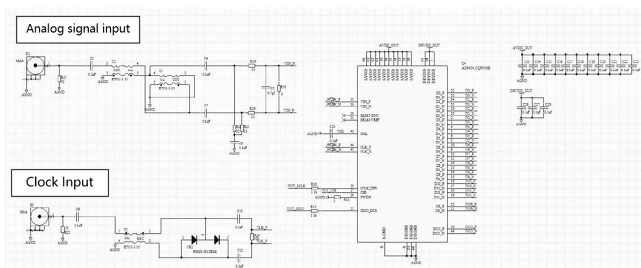
Figure 14. Typical Application Circuit
